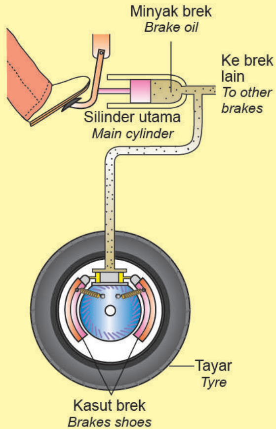
Brek hidraulik Hydraulic brakes
