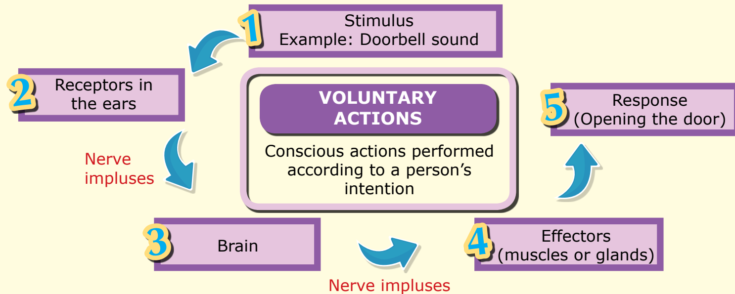
Pathway of impulses in voluntary actions
