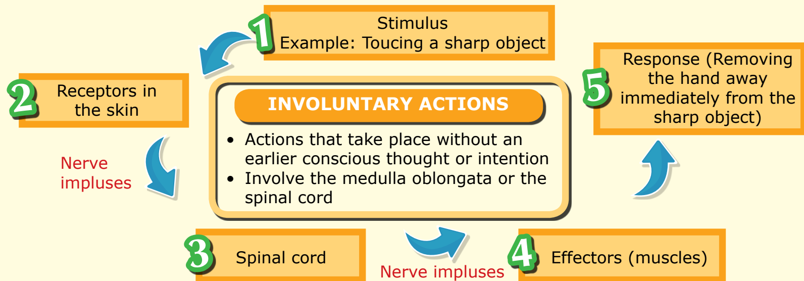
Pathway of impulses in involuntary actions (reflex actions)
