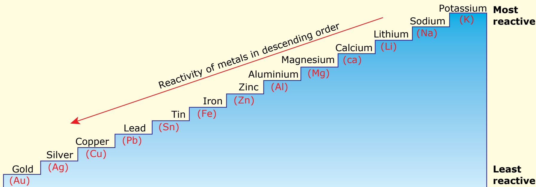
Reactivity Series of Metals
