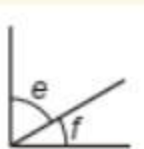
Sudut pelengkap Complementary angles e + f = 90^\circ
